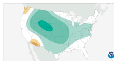
Outlook for Jun 2019 - Aug 2019 (Issued 16 May 2019) Higher chance of being wetter than usual Higher chance of being drier than usual Shaded areas show an increased chance of being higher or lower than usual during the next three months. The darker the shading, the greater the chance for the indicated condition. White areas have equal chances that are below, near, or above the long-term average (median) for the next three months. —Climate.gov
